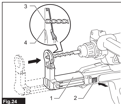
Fig.24 ► 1. Nozzle guide 2. Guide adjustment button 3. Tip of drill bit 4. Front surface of nozzle
