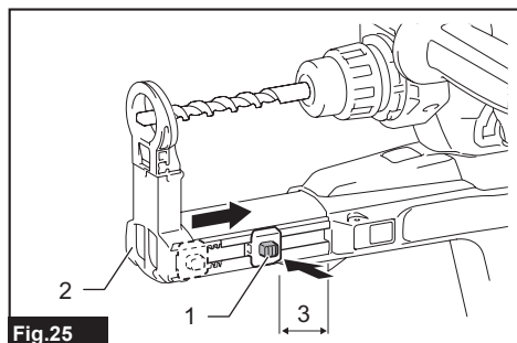
Fig.25 ► 1. Depth adjustment button 2. Nozzle guide 3. Drilling depths
