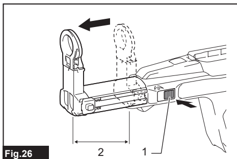
Fig.26 ► 1. Guide adjustment button 2. Approx. 100 mm (3-15/16")
